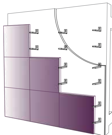
Figure-2: Direct fixing
