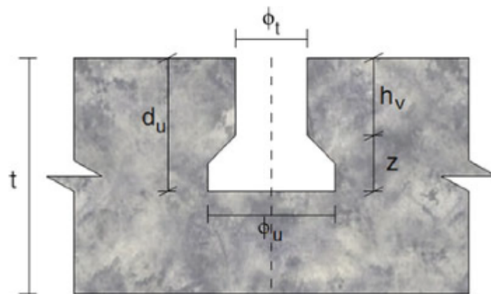
Figure: Dowel hole drilled in the back of the cladding material; (t) cladding material thickness, (du) dowel depth, (hv) fixed diameter depth, (z) variable diameter depth, ( \phi_t ) cylindrical dowel hole diameter, ( \phi_u ) undercut diameter
